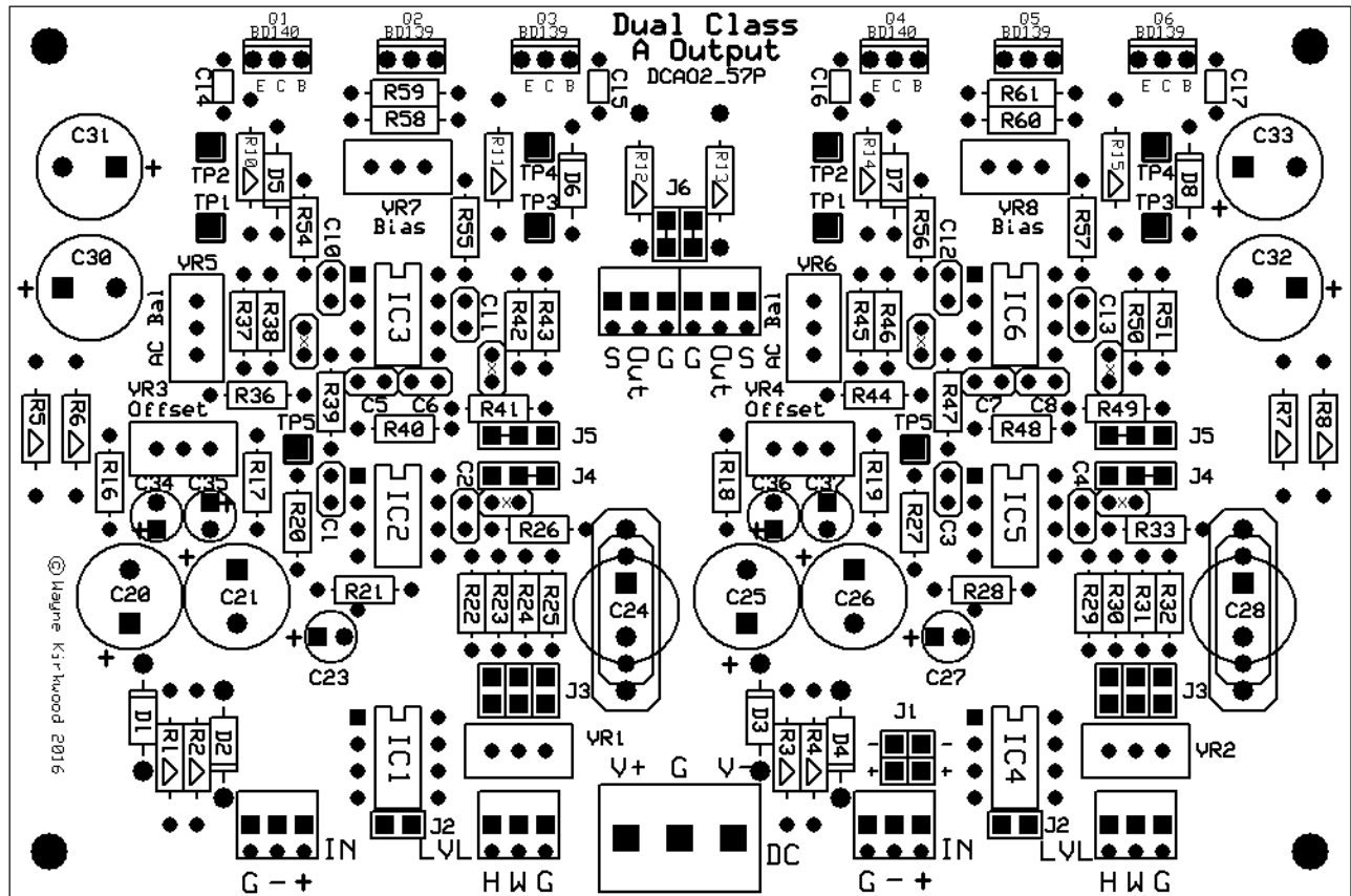
Dual Class-A PC Board Stuffing Guide
