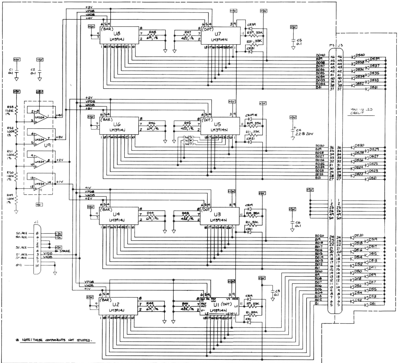
Bar and Peak Driver Circuits
