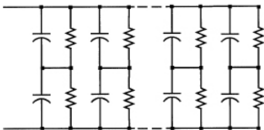
Series-parallel array, no center connection
