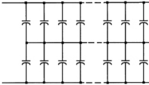
Parallel-series array with common center connection
