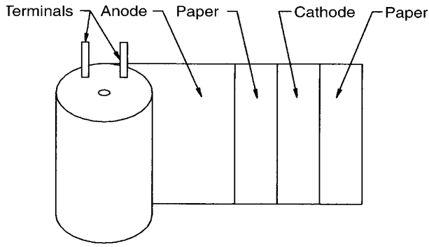
Wound Capacitor Elements
