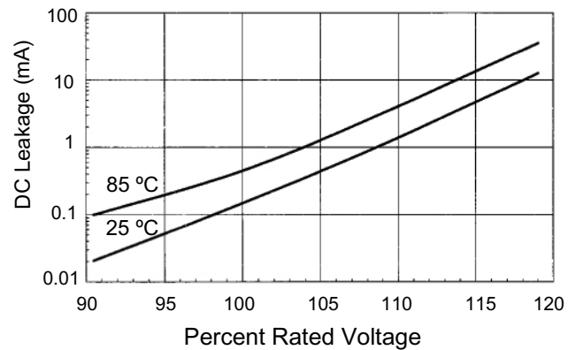
DC Leakage versus Voltage, 8600 \mu F 100 V
