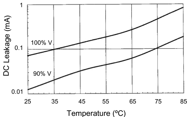
DC Leakage versus Temperature, 4700 \mu F 450 V
