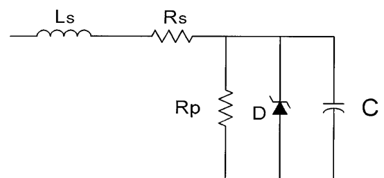
Equivalent Circuit
