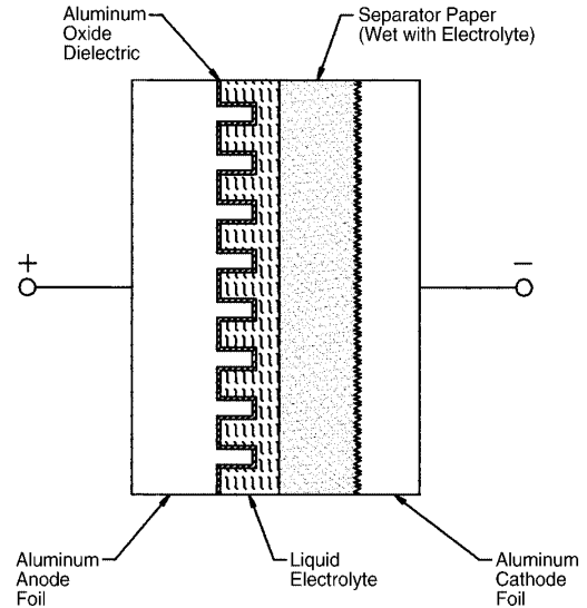
Capacitor-Element Materials
