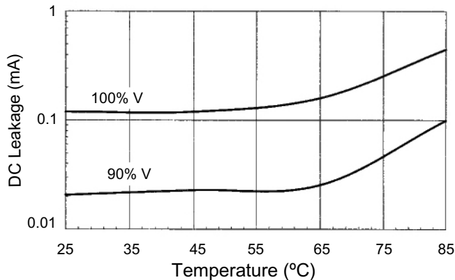
DC Leakage versus Temperature, 8600 \mu F 100 V
