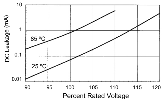
DC Leakage versus Voltage, 4700 \mu F 450 V
